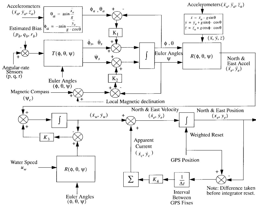
Fig. 2. Diagram of the SANS navigation filter.
