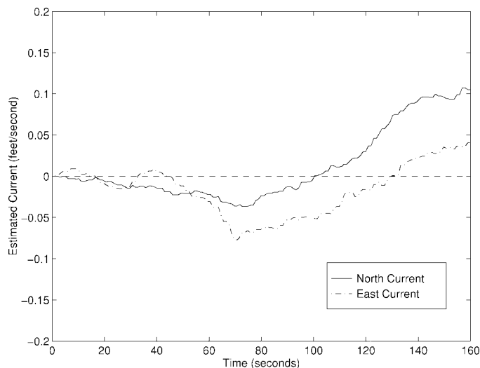
Fig. 5. Estimated current for bench testing with water speed being set to zero, K_1 = 0.1 , K_2 = 0.5 , K_3 = 2.0 , and K_4 = 0.01 .
